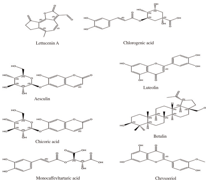
Figure 1. The chemical components of dandelion.
