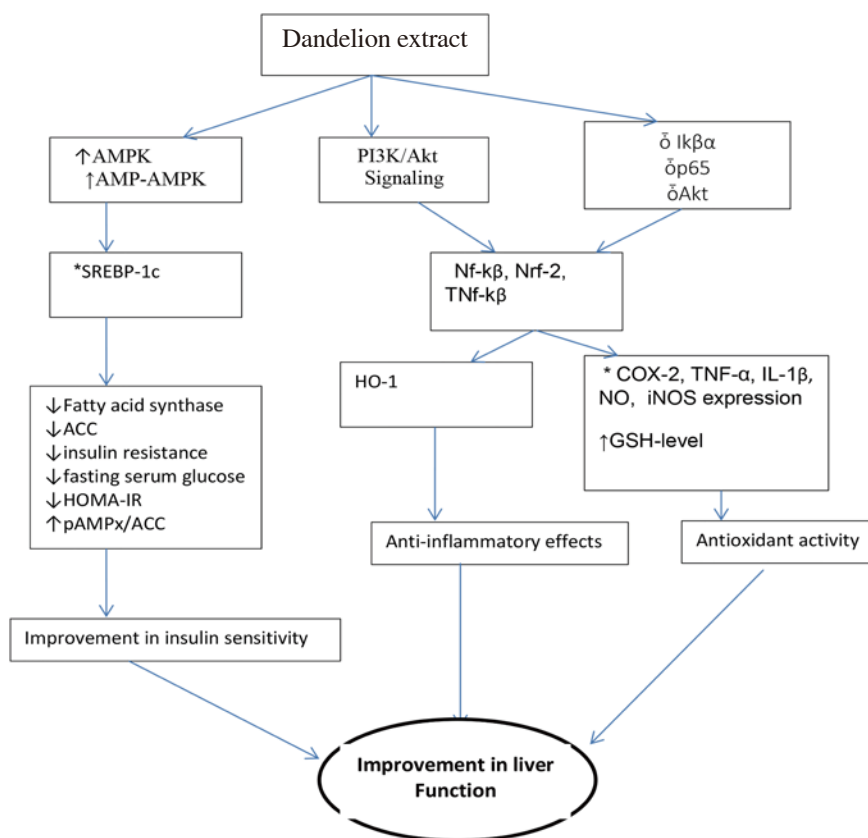
Figure 2. Molecular mechanism of hepatoprotective effects of dandelion.
